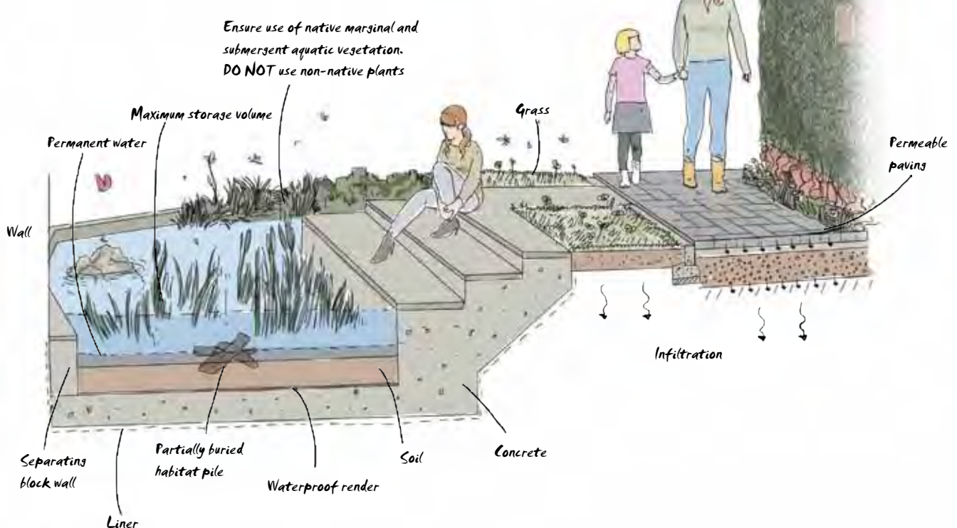
Figure 11 Urban ponds integrated into hard landscaping of SuDS can provide somewhere pleasant to sit, and when planted appropriately can also be attractive to wildlife.
