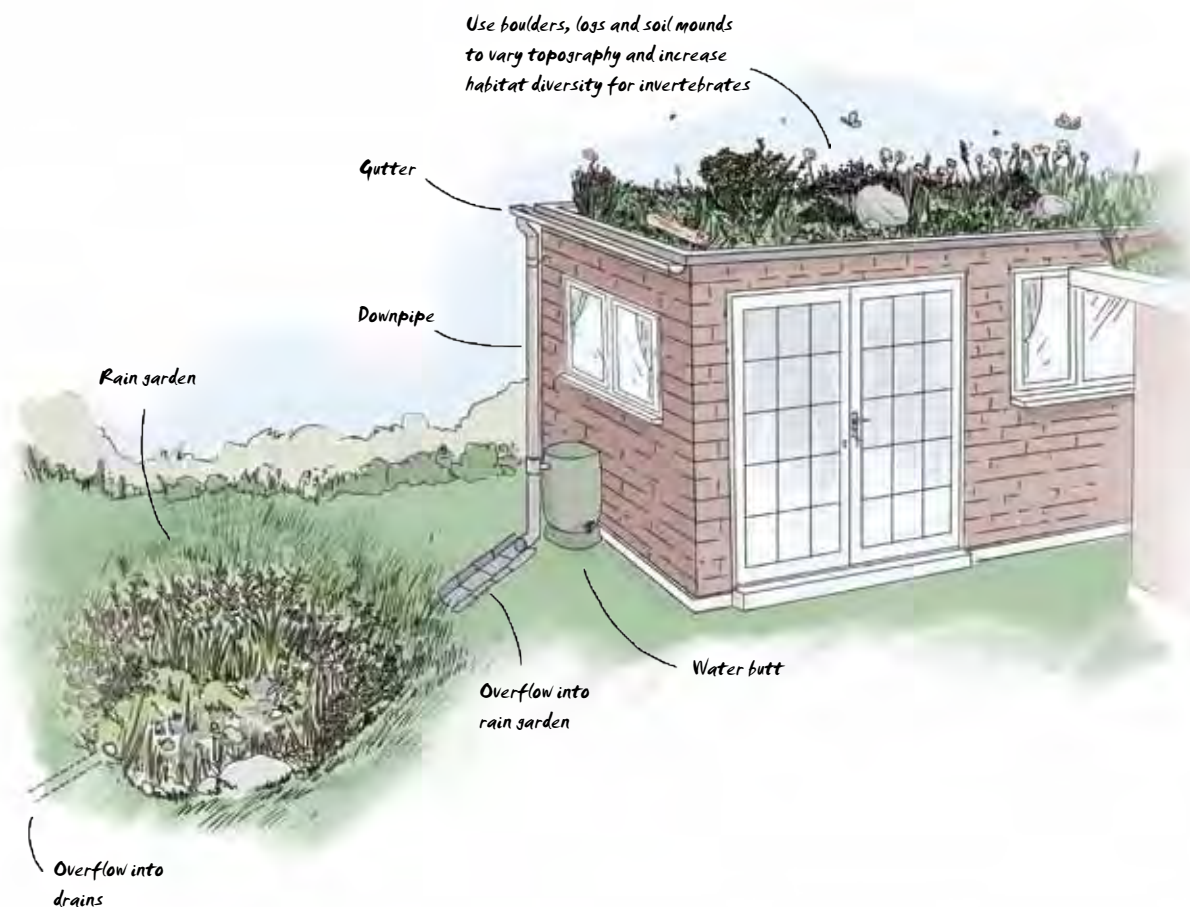
Figure 5 Extensive green roof linked to a rain garden via a water butt.
