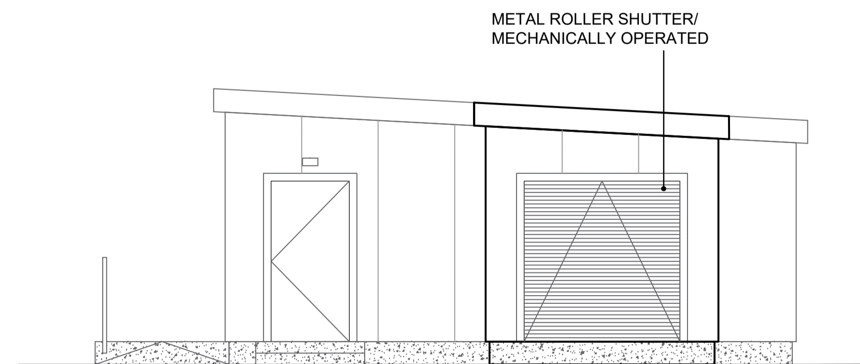
ELEVATION C
