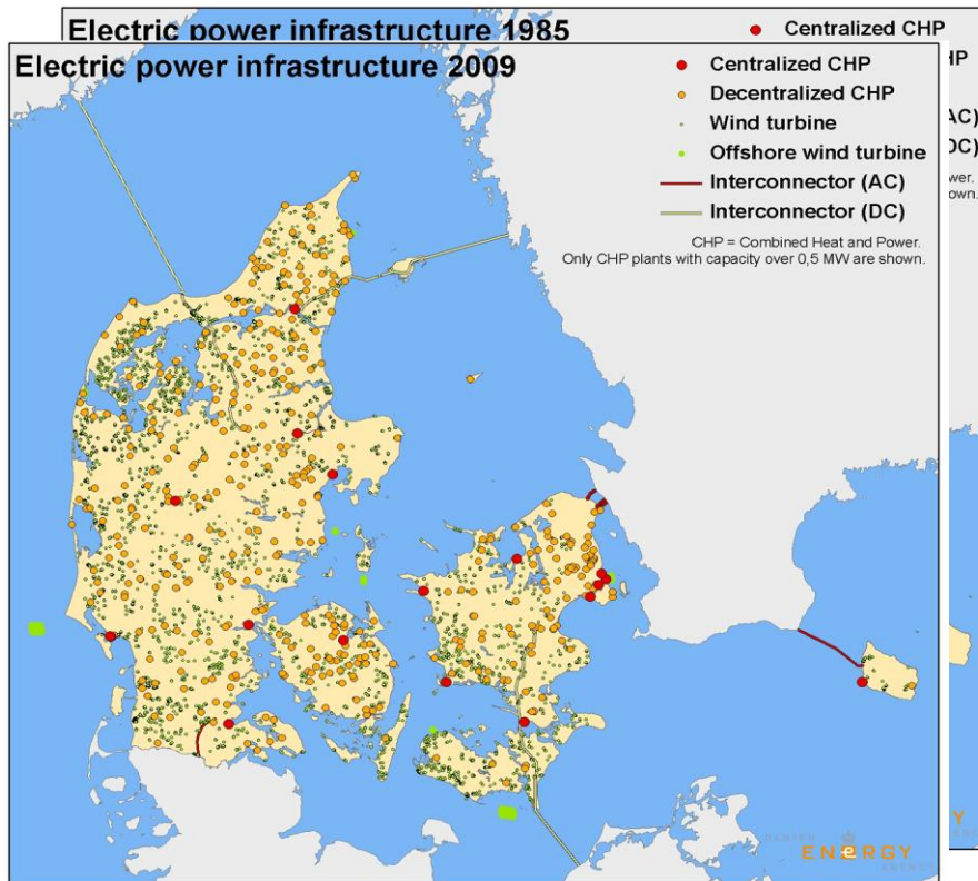
Figure 3: Denmark's Electricity Infrastructure 1985 and 2009 98
